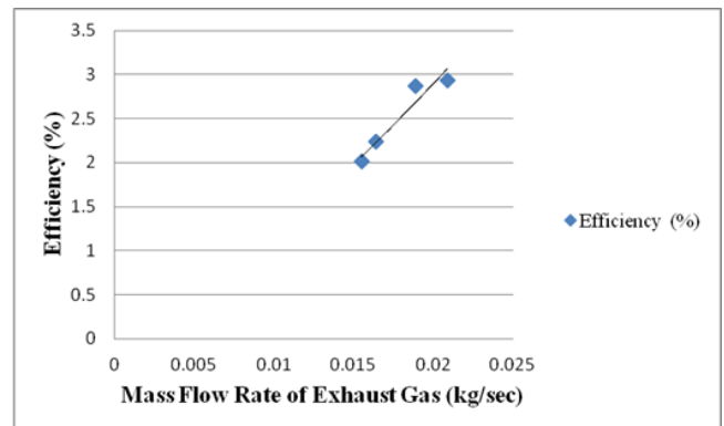
Fig. 7. Effect of mass flow rate of exh. gas on efficiency
