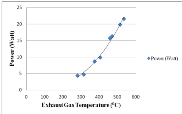
Fig. 4. Effect of exhaust gas temperature on output Power
