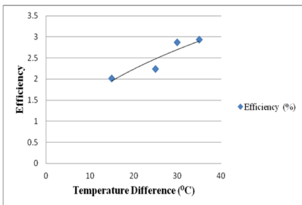
Fig. 6. Effect of temperature difference on efficiency
