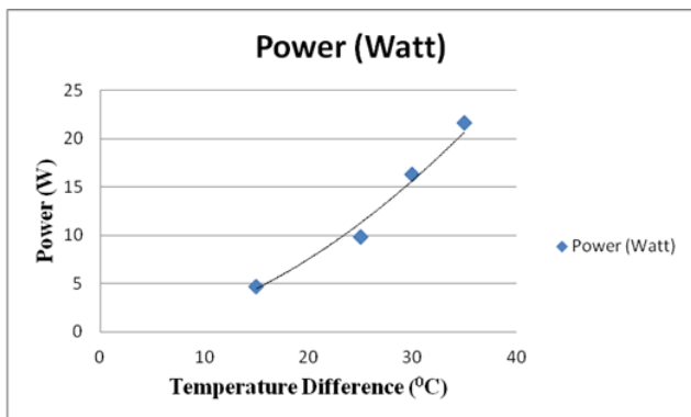
Fig. 5. Effect of temperature difference on output Power
