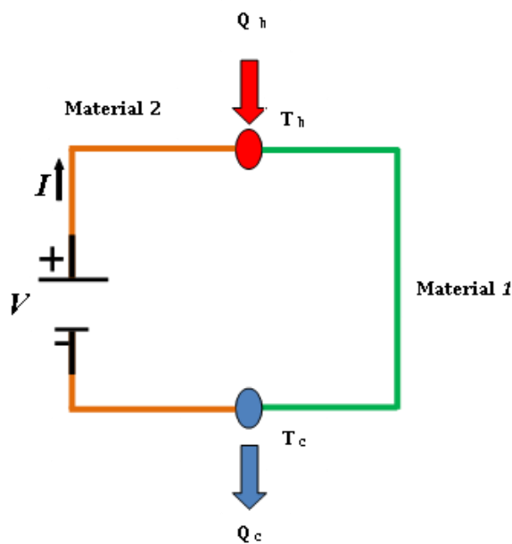
Fig. 1. Schematic of the Seebeck effect represented on a thermocouple
