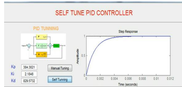
Fig. 2. Step response of the proposed system at auto tuned PID gain parameters
