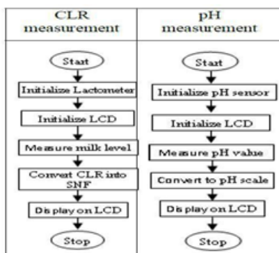
Fig. 5. Processing and Display (Flow chart)
