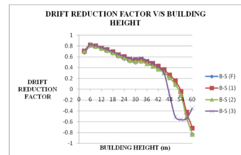
Fig. 9. 20 Storied building (Dynamic Analysis)
