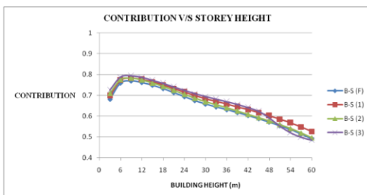
Fig. 11. 20 Storied building (Dynamic Analysis)
