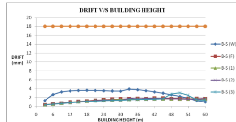
Fig. 6. 20 Storied building (Static Analysis)
