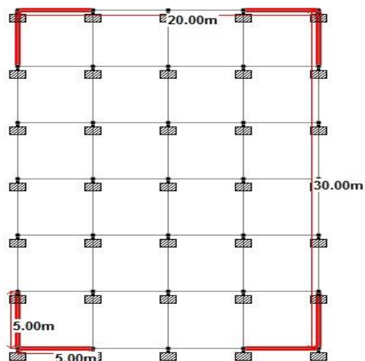
Fig. 3. Plan of building with position of shear wall
