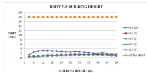
Fig. 7. 20 Storied building (Dynamic Analysis)
