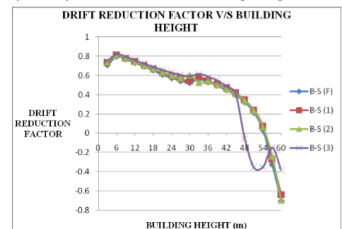
Fig. 8. 20 Storied building (Static Analysis)
