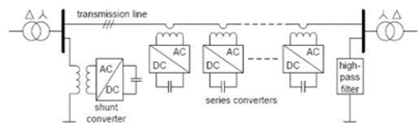
Fig. 2. DPFC Configuration
