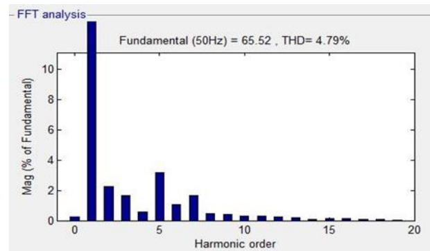
Fig. 13. Current THD
