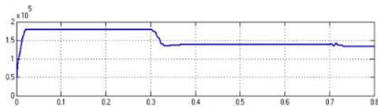
Fig. 7. Reactive power at Bus-2
