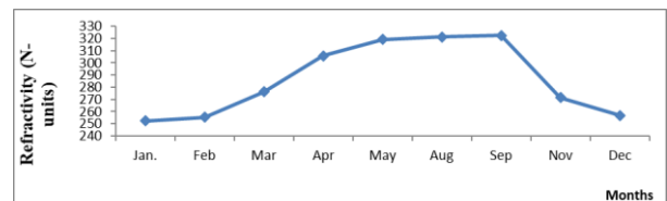
Fig. 10. Variation of mean refractivity from January to December of year 2014
