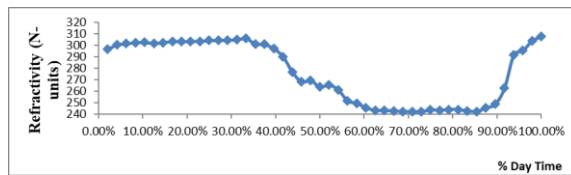
Fig. 3. Variation of refractivity with % time of the day month of March
