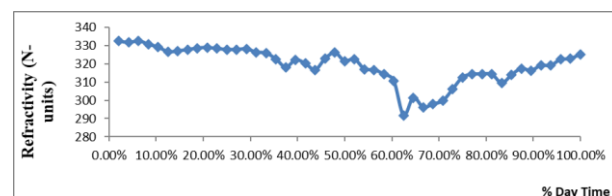
Fig. 5. Variation of refractivity with % time of the day month of May
