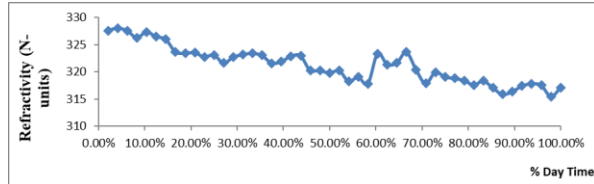
Fig. 6. Variation of refractivity with % time of the day month of August
