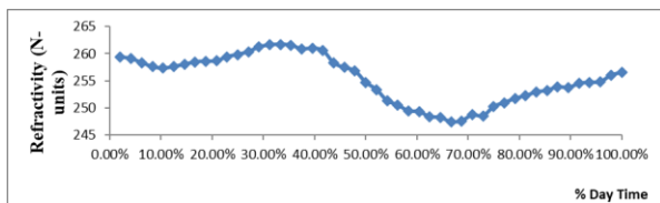
Fig. 2. Variation of refractivity with % time of the day month of February
