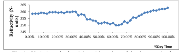
Fig. 9. Variation of refractivity with % time of the day month of December
