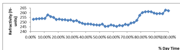
Fig. 1. Variation of refractivity with % time of the day month of January
