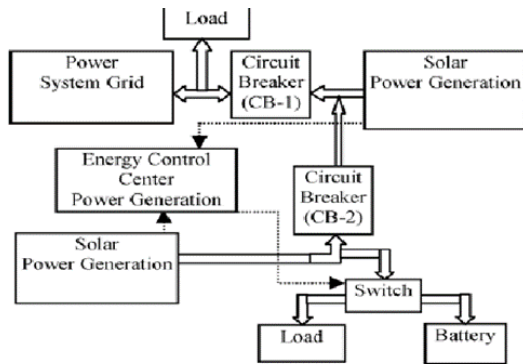
Fig. 1. Block diagram of ECC
