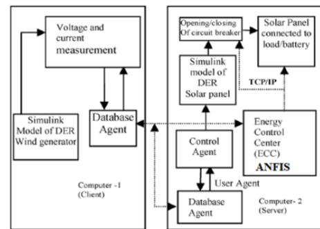
Fig. 2. Operation of multi-agent
