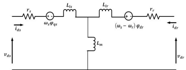
Fig. 2. d-axis equivalent circuit of WRIM
