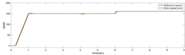
Fig. 8. Rotor speed tracking using fuzzy logic controller
