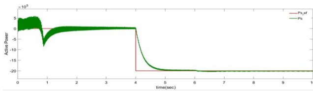
Fig. 9. Active power of stator using PI Controller
