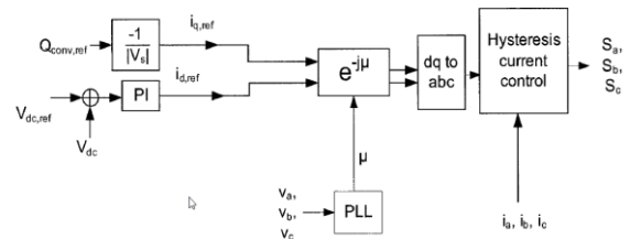
Fig. 5. Grid side converter control for regulation of dc voltage and supply of reactive power
