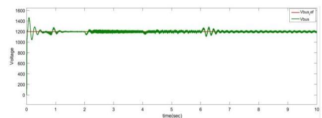
Fig. 14. DC link bus voltage for fuzzy logic Controller
