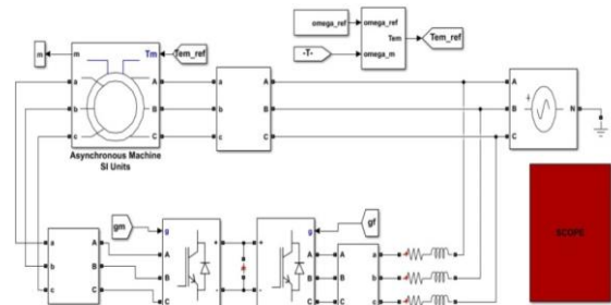
Fig. 6. Simulink diagram of doubly fed induction generator
