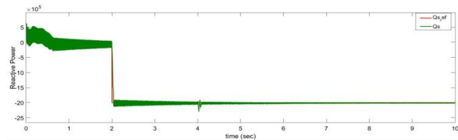
Fig. 12. Reactive power of stator using fuzzy controller
