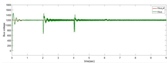
Fig. 13. DC link bus voltage for PI Controller
