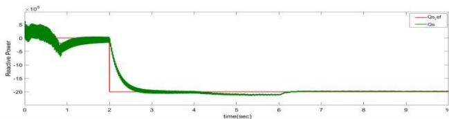
Fig. 11. Reactive power of stator using PI controller
