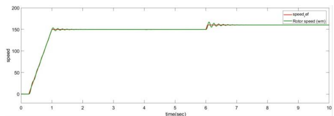
Fig. 7. Rotor speed tracking using PI controller
