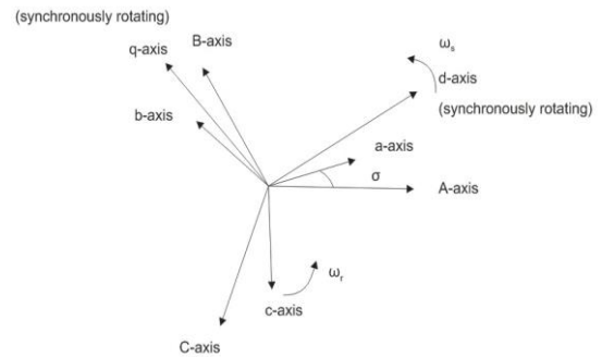
Fig. 1. Reference system used in DFIG
