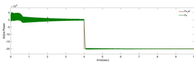
Fig. 10. Active power of stator using Fuzzy Logic Controller
