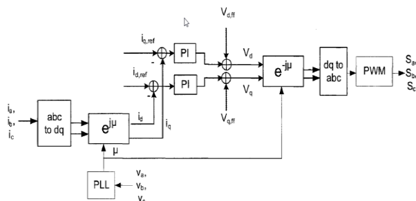
Fig. 4. PWM linear feedback current control scheme
