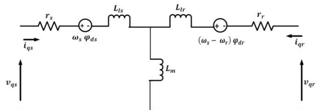
Fig. 3. q-axis equivalent circuit of WRIM
