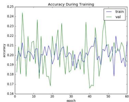
Fig. 12. Training and validation accuracy for the CNN
