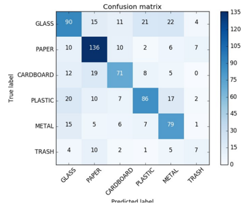
Fig. 9. Confusion matrix from the SVM run on a smaller version of the dataset
