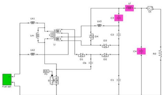
Fig. 4. Simulation circuit
