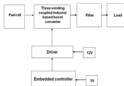
Fig. 1. Block diagram
