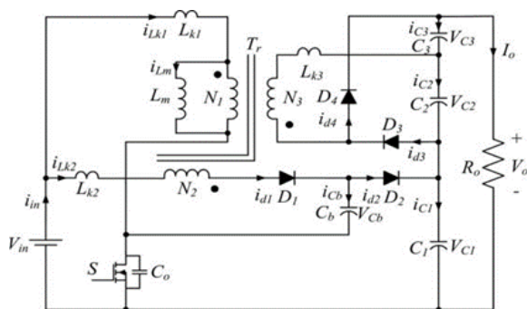
Fig. 2. Circuit diagram
