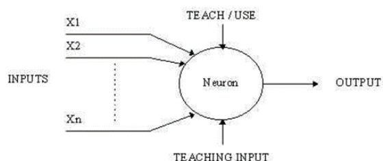
Fig. 2. Artificial neuron [11]
