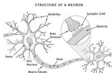
Fig. 1. Biological neuron [10]
