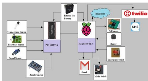
Fig. 2. Architecture diagram
