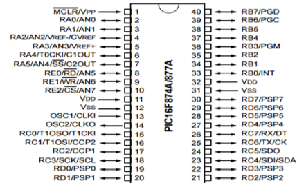
Fig. 5. Pin diagram of 16F877A
