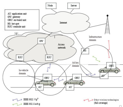
Fig. 2. Research issues
