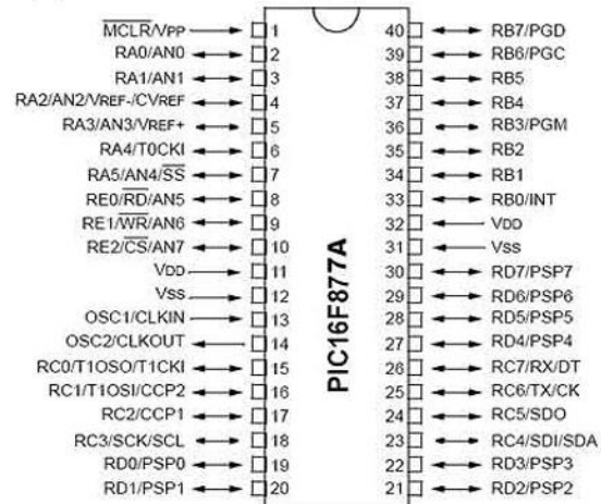
Fig. 2. Pin diagram of PIC16F877A
