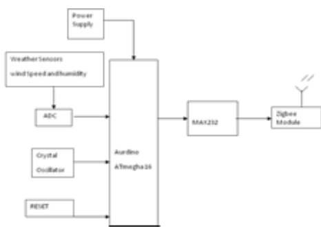
Fig. 1. Transmitter Circuit.
