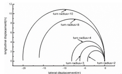
Fig. 8. Locus of different turn radius achieved by skid steering
