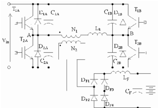
Fig. 5. The H-bridge converter for charger
