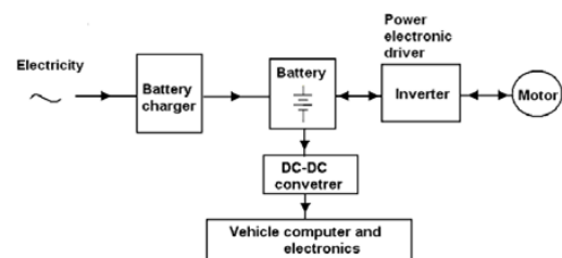
Fig. 2. The key components of an Electric Vehicle.
