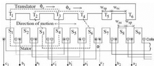
Fig. 9. Active suspension based on linear motor.
