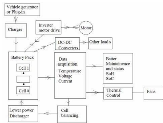
Fig. 6. Schematic of the BMS
