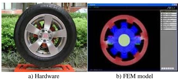
Fig. 3. The in-wheel motor
